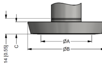
dairy pipe (DIN 11851)
