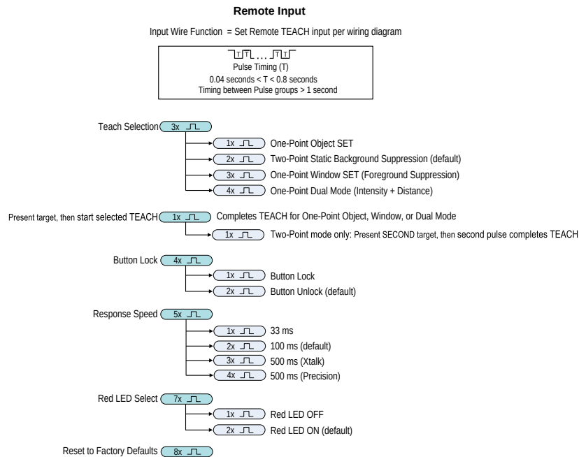
Figure 6. Remote Input menu
