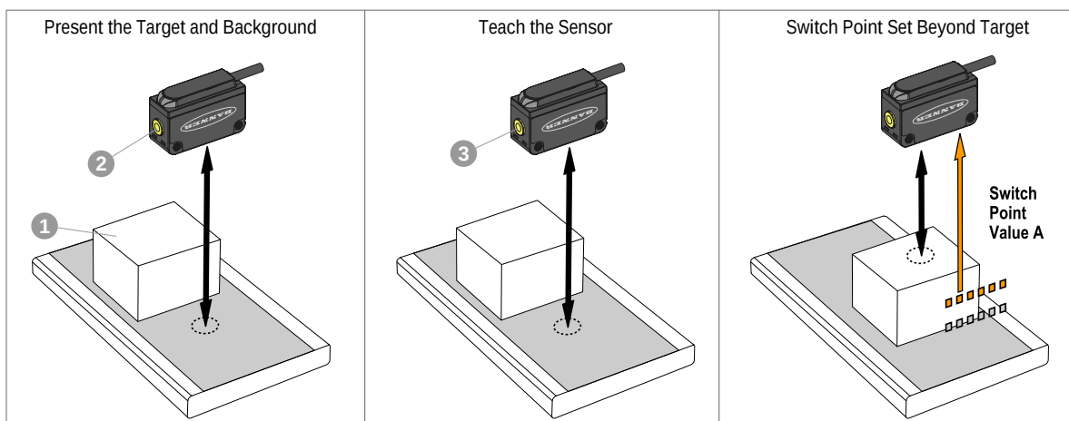
Figure 7. TEACH Process for Two-Point Static Background Suppression
