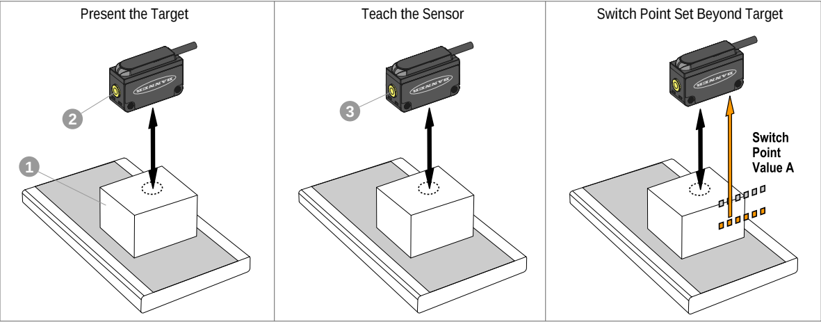
Figure 8. TEACH Process for One-Point Object SET
