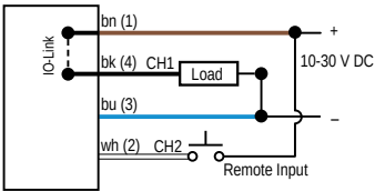
Figure 2. CH1 as PNP/IO-Link and CH2 as the Remote Input
