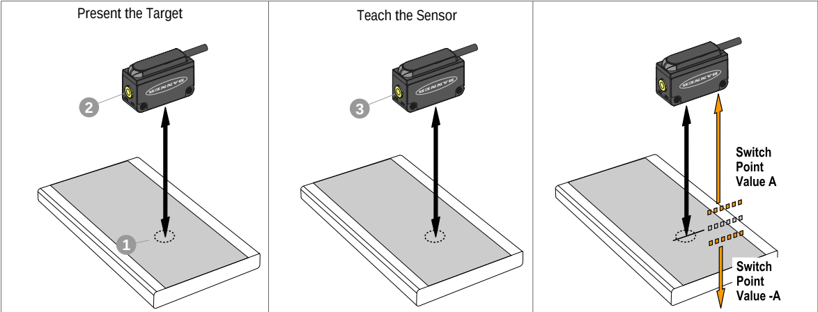
Figure 9. TEACH Process for One-Point Window SET (FGS)
