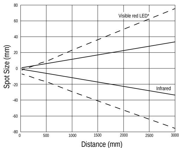
Figure 11. Spot Size
