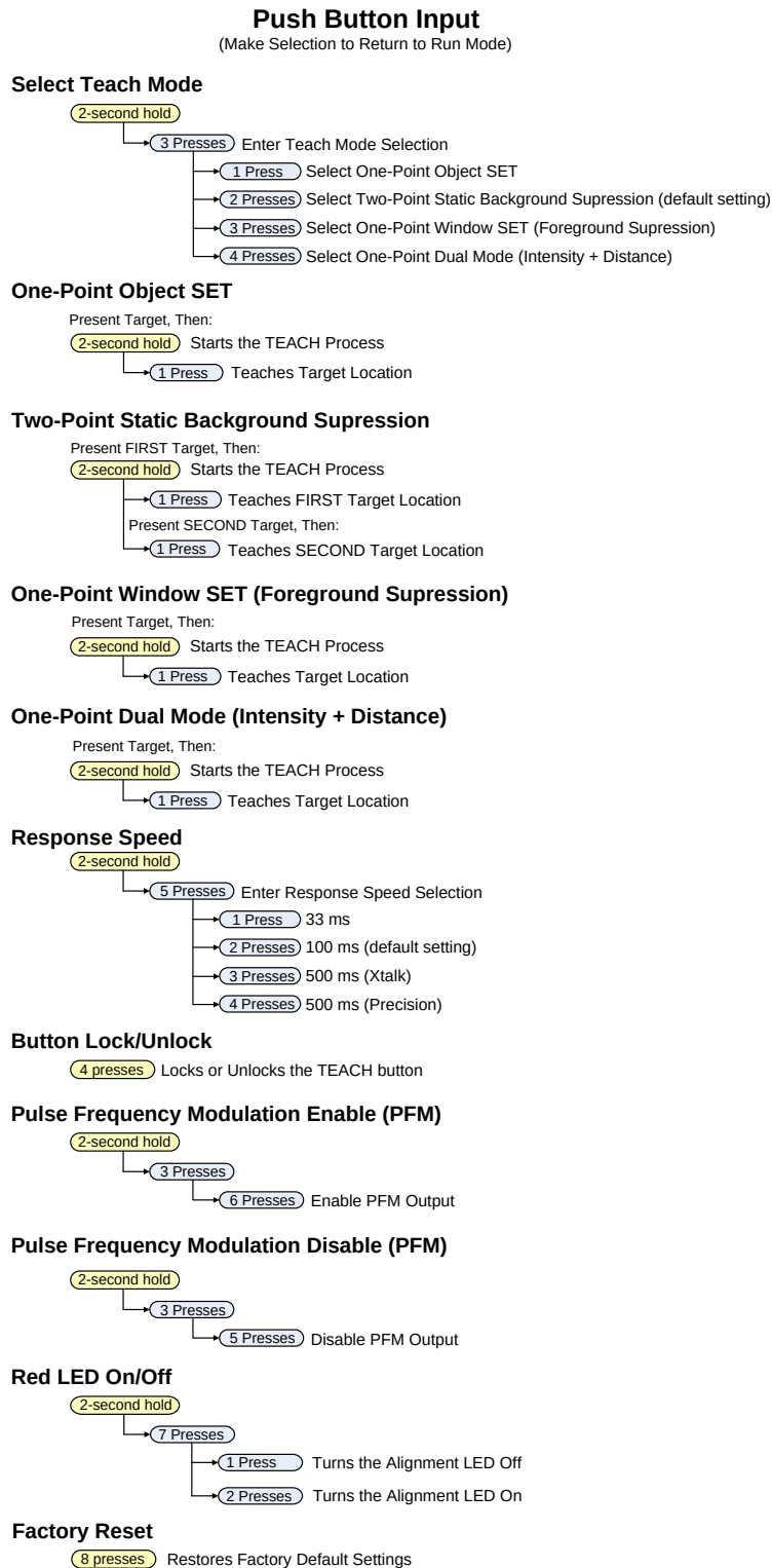
Figure 5. TEACH Button Chart
