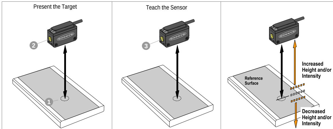
Figure 10. TEACH Process for One-Point Dual Mode
